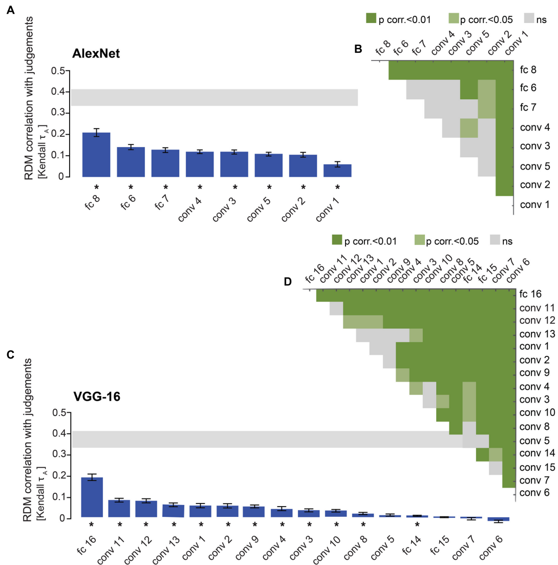
FIGURE 6 | DNN performance at explaining similarity judgments: late layers outperform early layers. (A) Bars show the correlation between the similarity-judgment RDMs and each fitted AlexNet layer RDM. Noise ceiling and significant correlations are indicated using the same conventions as in Figure 4 . (B) Pairwise differences between model performance of fitted AlexNet layer RDMs, using the same conventions as in Figure 4 . (C) Bars show the correlation between the similarity-judgment RDMs and each fitted VGG-16 layer RDM. (D) Pairwise differences between model performance of fitted VGG-16 layer RDMs.
