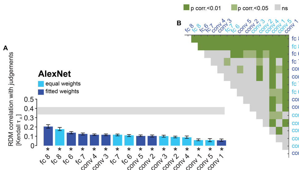
FIGURE 4 | AlexNet performance at explaining similarity judgments: reweighting improves model performance for late layers. (A) Bars show the correlation between the similarity-judgment RDMs and each AlexNet layer RDM, with and without reweighting. A significant correlation between a layer RDM and the similarity-judgment RDMs is indicated by an asterisk (one-sided Wilcoxon signed-rank test, p < 0.05 corrected). Error bars show the standard error of the mean based on single-subject correlations, i.e., correlations between the single-subject similarity-judgment RDMs and a DNN RDM. The gray bar represents the noise ceiling, which indicates the expected performance of the true model given the noise in the data. “conv” indicates a convolutional layer and “fc” indicates a fully-connected layer. (B) Pairwise differences between model performance of AlexNet layer RDMs, with and without reweighting. Green color indicates significant pairwise differences (dark green p < 0.01 , light green p < 0.05 , FDR corrected across all comparisons).
