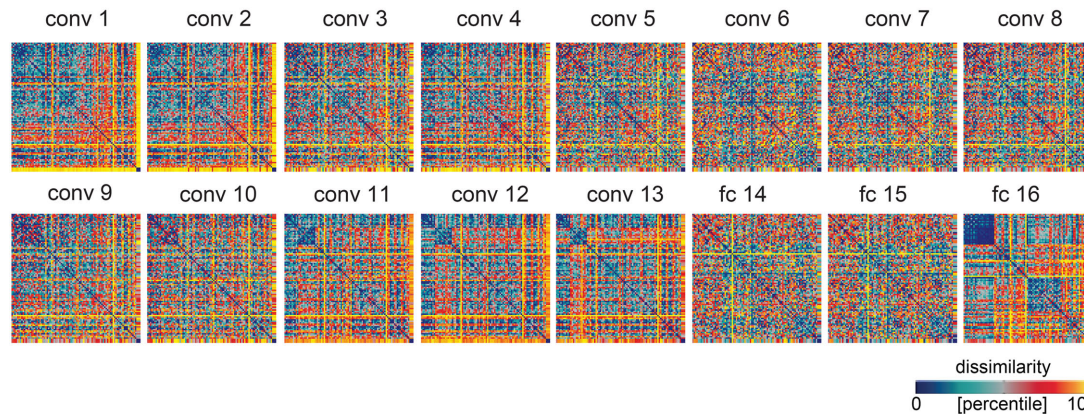
FIGURE 3 | Model predictions of the similarity judgments for each DNN layer. RDMs for each layer of each network, after weighting the feature maps (convolutional layers) or model units (fully-connected layers) within that layer to best predict the human similarity judgments. Values within each RDM were transformed into percentiles for visualization (see color bar).
